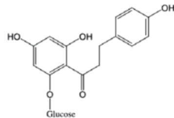
Florizin
