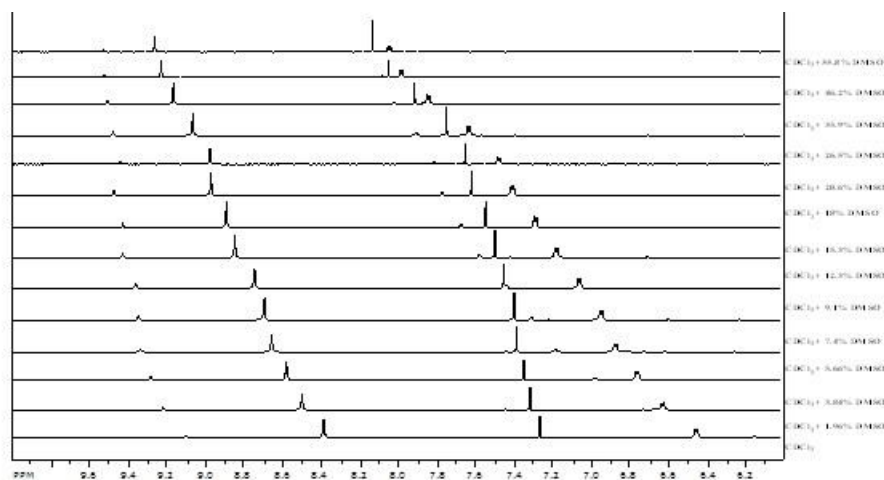
4 (Ac-L-Ala-D-Pro-NH-Fca-COOMe)
