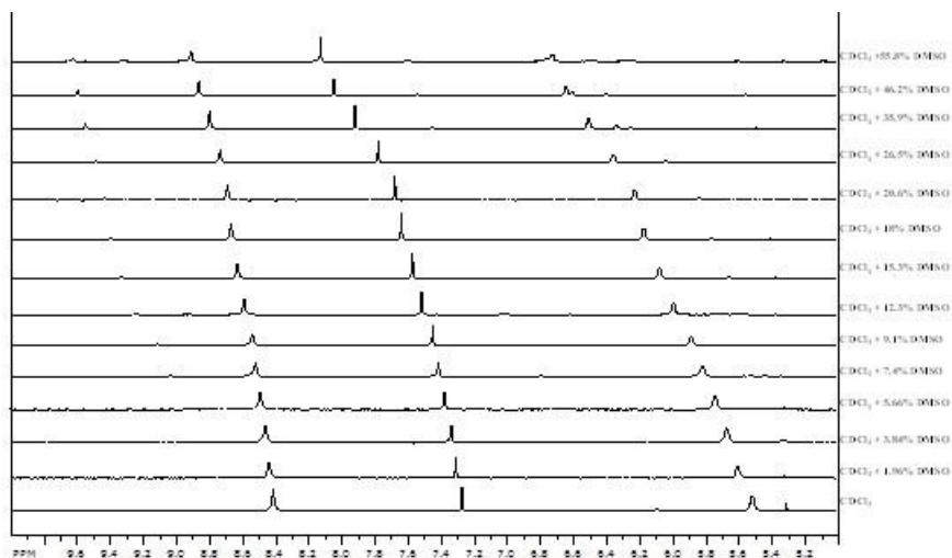
2 (Boc-L-Ala-D-Pro-NH-Fca-COOMe)
