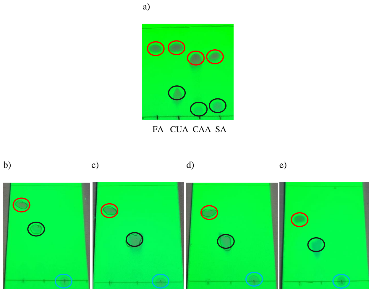
Figure 7. a) TLC of reaction mixtures (Rm) one hour after starting the decarboxylation reactions of p -CUA, CAA and FA (2.5 mM each) catalyzed by BsPAD wt (0.005 μg/mL) and SA (2.5 mM) catalyzed by BsPAD I85A (0.01 μg/mL). TLC of Rm three hours after starting decarboxylation reaction of: (b) p -CUA, (c) CAA and (d) FA by BsPAD wt . TLC of Rm three hours after starting decarboxylation reaction of SA by BsPAD I85A . Spots highlighted with red circles represent decarboxylated products 4-VP, 4-VC, 4-VG and 4-VS. Black circles represent 10 mM substrate standards ( p -CUA, CAA, FA and SA), and blue circles represent BsPAD wt or BsPAD I85A enzyme dilution, also serving as standards
