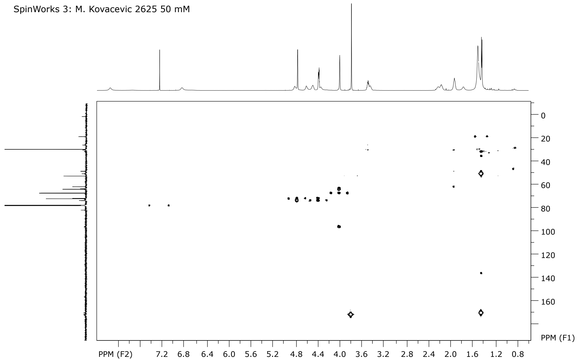
Figure S32. ^1\text{H} - ^{13}\text{C} HMBC spectrum of compound 4 ( c = 5 \times 10^{-2} M).
