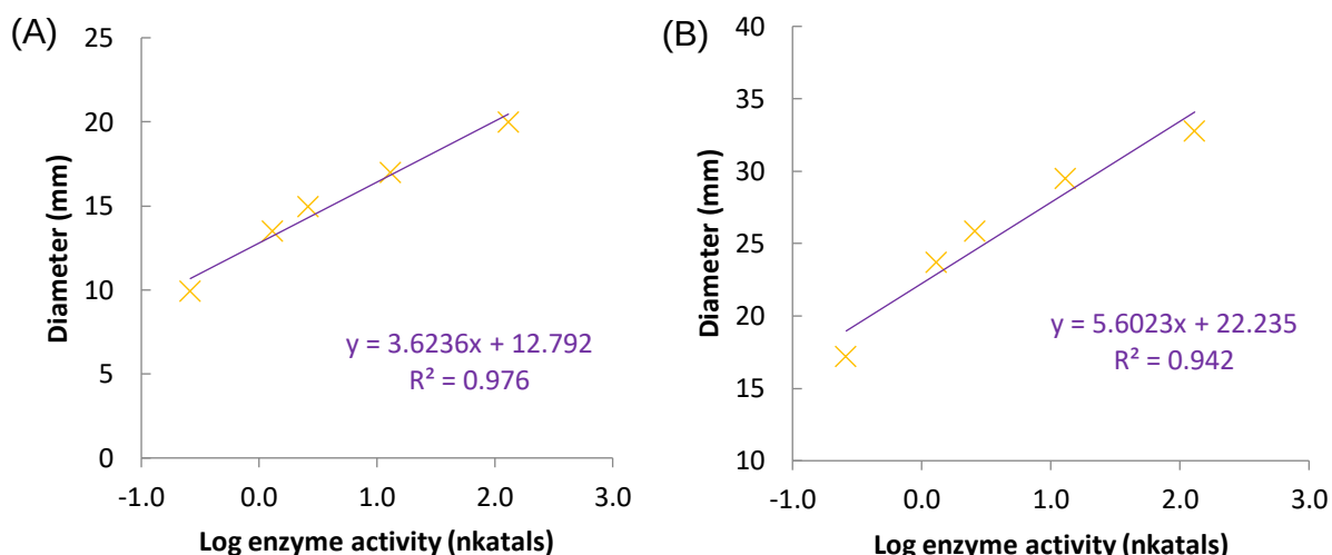
Figure 7. Standard curve showing the dependence of hallos diameter (mm) corresponding to demetylestirified pectin and the logarithmic value of the commercial PME activity (nkatal) at (A) pH5 (B) pH7.6.
