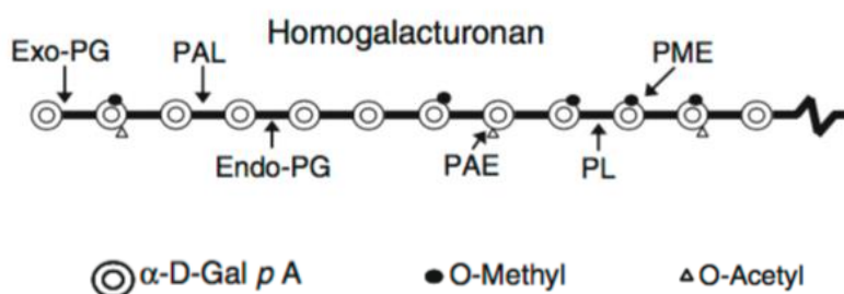
Figure 3. Mode of action of pectinases involved in the degradation of homogalacturonans. Exo-PG: exopolygalacturonases, PAL: pectate lyases, Endo-PG: endopolygalacturonases, PAE: pectin acetyl esterases, PL: pectin lyases, PME: pectin methyl esterases. Figure has been adapted from Hilz, 2007.
