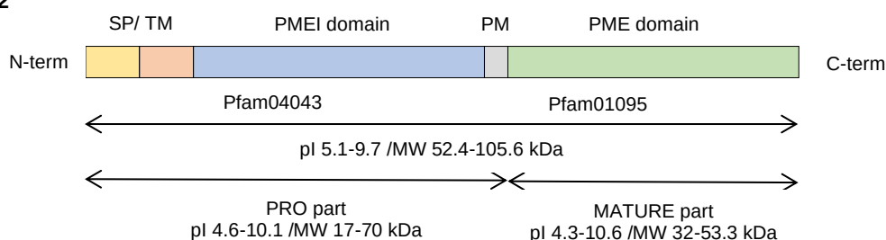
Figure 5. Differences in the protein structure between Group 1 and 2 PMEs. All PME proteins (Group 1 and 2) have conserved PME domain (Pfam01095) and signal peptide/ transmembrane domain (SP/TM), while only proteins from Group 2 have PRO region which shares similarities with the PMEI domain (Pfam04043) and a processive motifs (PM). Figure adapted from Pelloux et al. , 2007.
