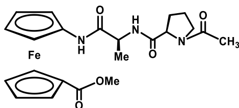
Ac-D-Pro-L-Ala-NH-Fn-COOMe (4)
