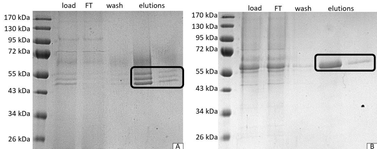
Figure 7. 12 % SDS PAGE, stained with Coomassie blue, of AtPGAZAT (A) and AtPGLR (B) with samples from different steps of purification.
