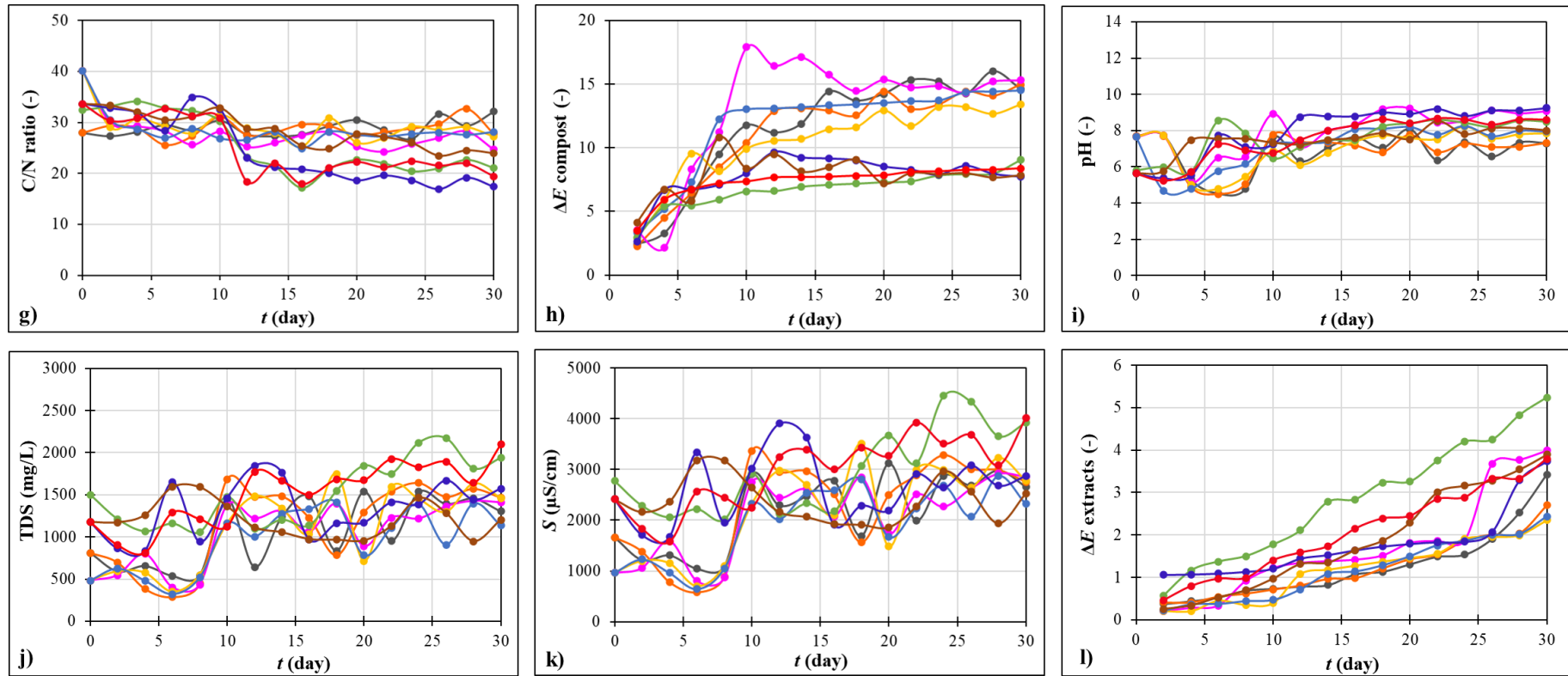
Figure 15. (continuing) Changes in g) C/N ratio; h) \Delta E compost; i) pH; j) TDS; k) S and l) \Delta E extracts during the 30 days of grape skin composting process ( \bullet experiment 1; \circ experiment 2; \blacklozenge experiment 3; \blacktriangle experiment 4; \blacktriangledown experiment 5; \blacktriangleright experiment 6; \blacktriangleleft experiment 7; \blacktriangleright experiment 8; \blacktriangleleft experiment 9) ( \Delta E compost=total color change of compost samples; TDS=total dissolved solids; S =conductivity; \Delta E extracts=total color change of compost extracts)
